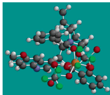
Figure 3. PM3-based model of metal enolate binding in complex 12a showing expected si -face selectivity.
