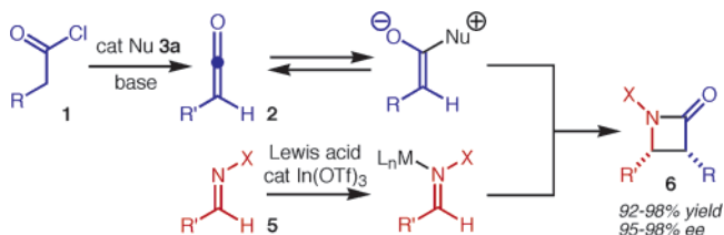
Scheme 1. Tandem Lewis Acid/Nucleophile Catalyzed Synthesis of \beta -Lactams
