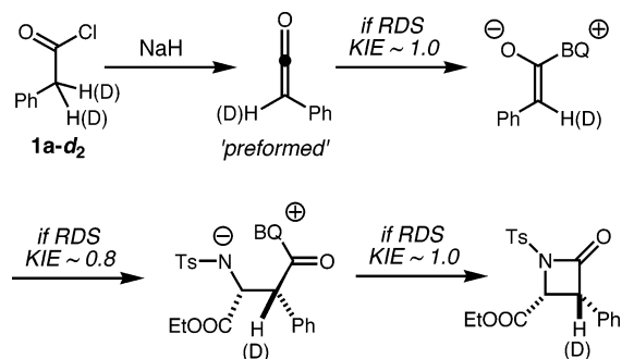
Scheme 4. Kinetic Isotope Study To Identify the Rate-Determining Step
