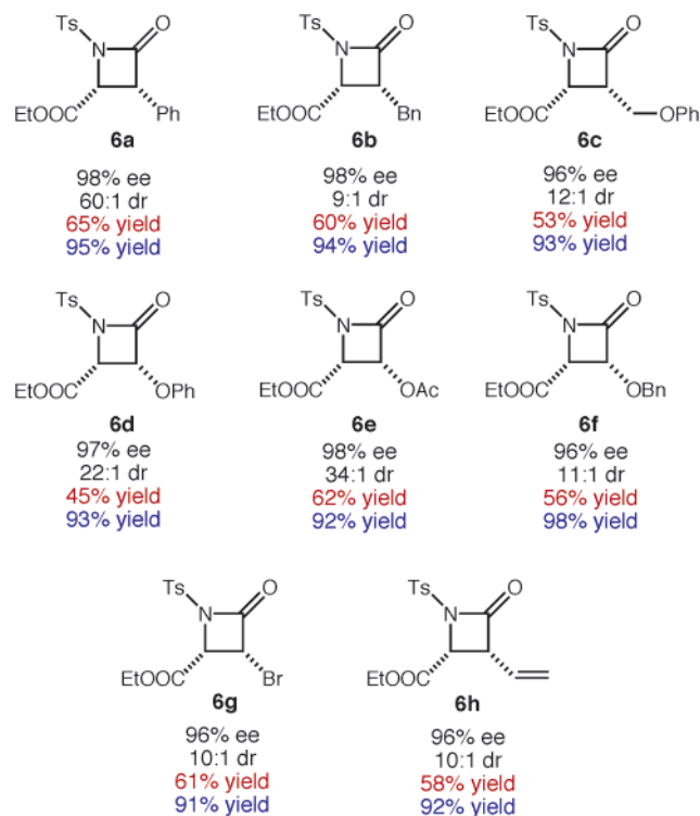
Figure 1. \beta -Lactams synthesized by employing BQ and In(OTf) 3 cocatalyst. 23
