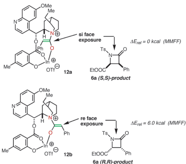
Figure 2. Expected facial discrimination of indium complex 12 for intramolecular bifunctional activation.
