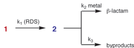
Scheme 3. Metal-Mediated Bifurcated Pathway for the Formation of \beta -Lactams
